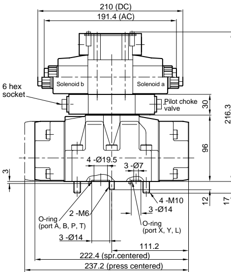
3 POSITION VALVE
