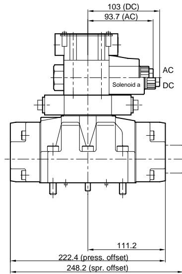
2 POSITION VALVE
