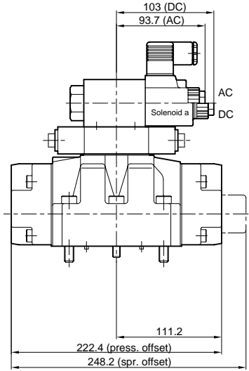
2 POSITION VALVE
