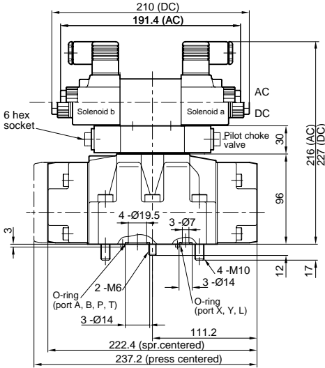
3 POSITION VALVE
